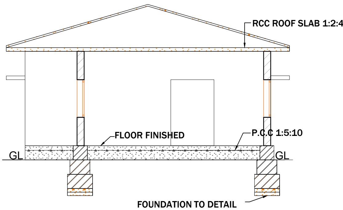
SECTION "A-B"
