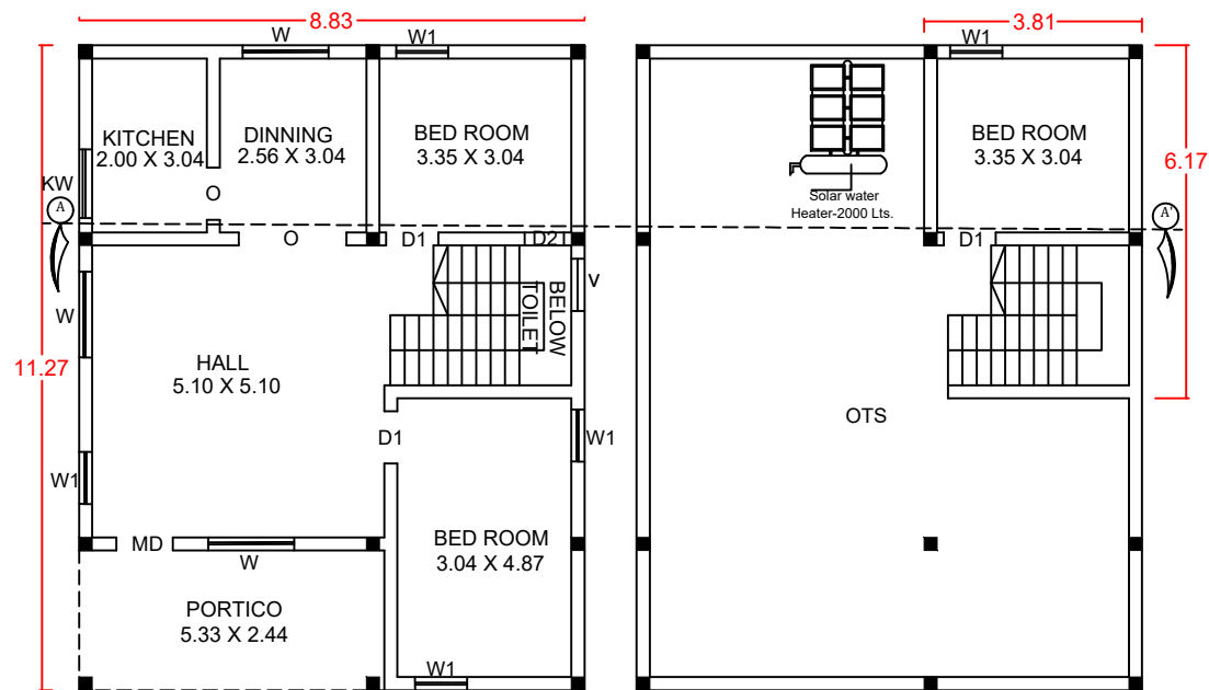
GROUND FLOOR
