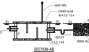
SECTION-A-B
