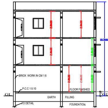
SECTION "A-B"
