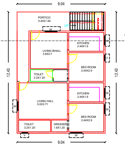
PRO.SECOND FLOOR PLAN SCALE:1:100
