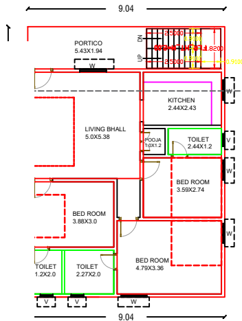
EXI.FIRST FLOOR PLAN SCALE:1:100
