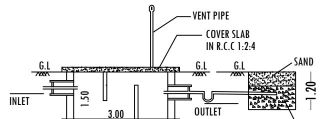
SECTION-AB
