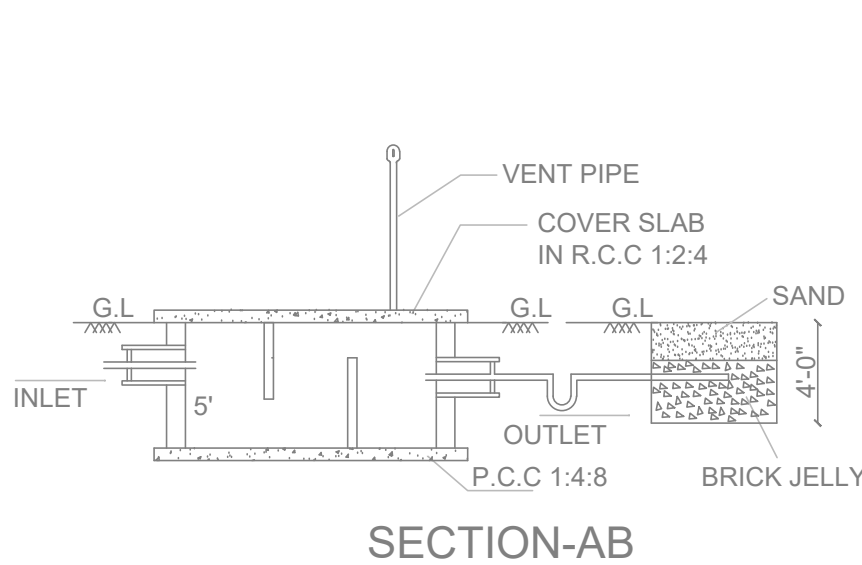
SECTION-AB
