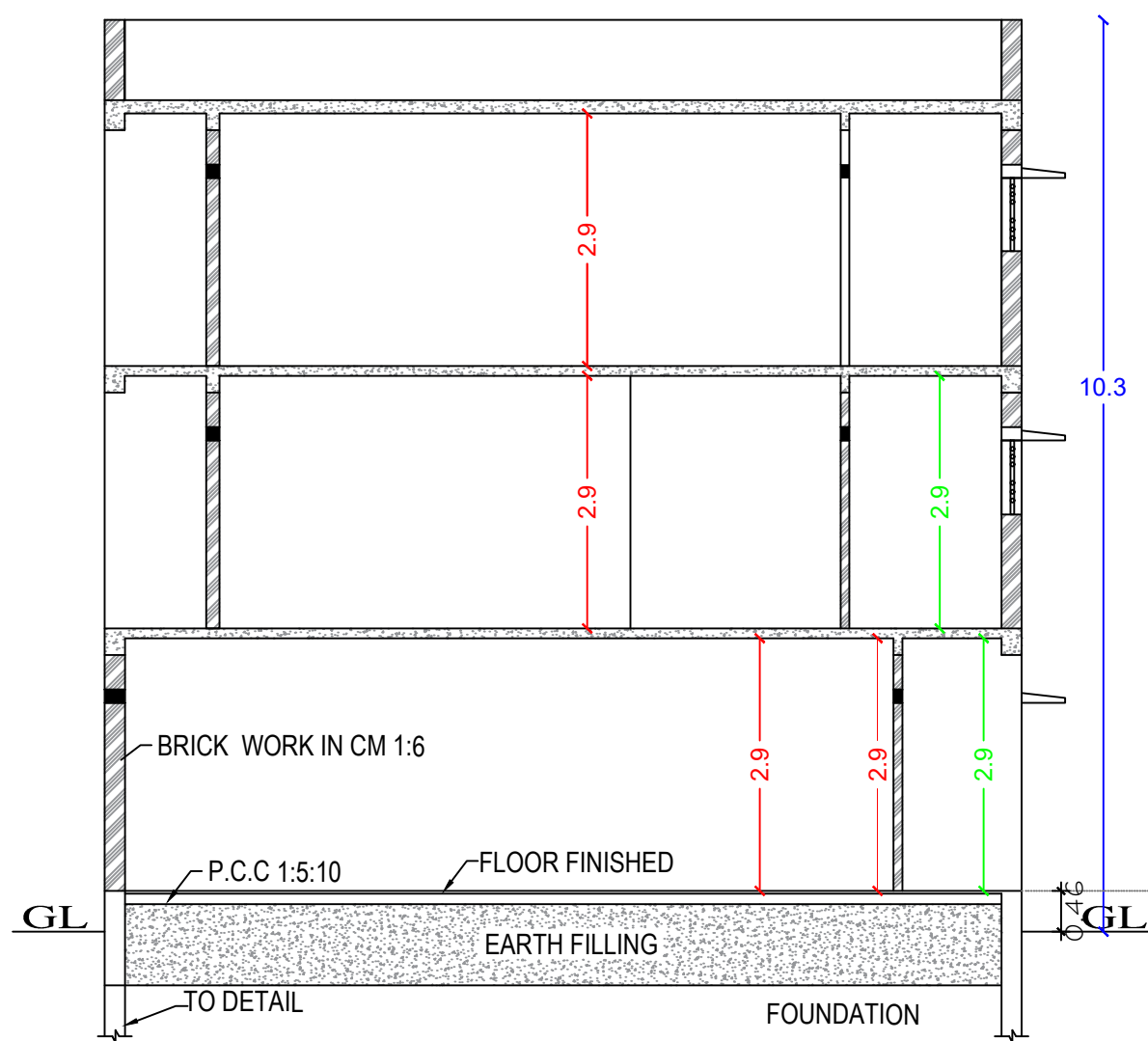
SECTION "A-B"
