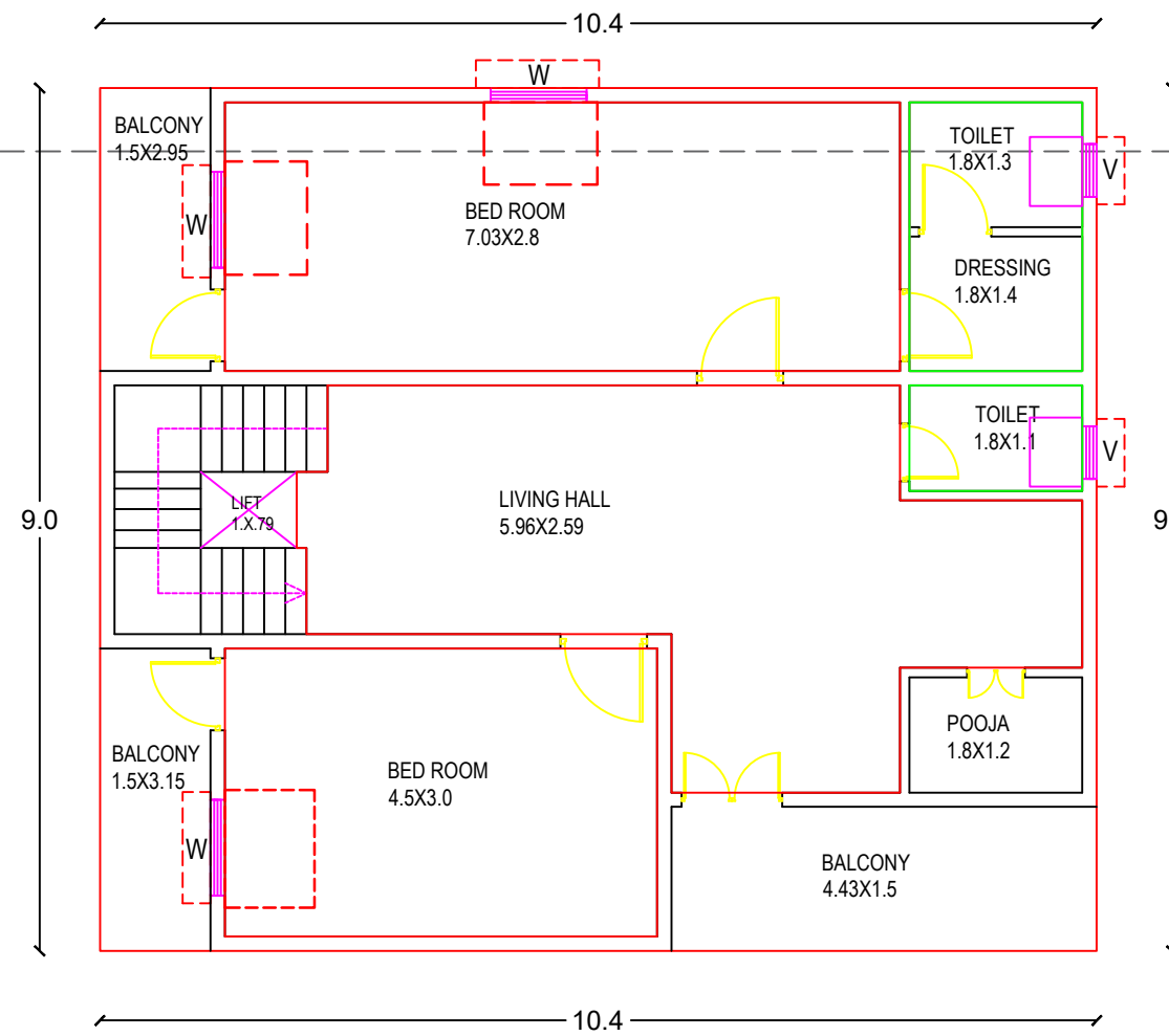
PRO.FIRSTS FLOOR PLAN SCALE:1:100
