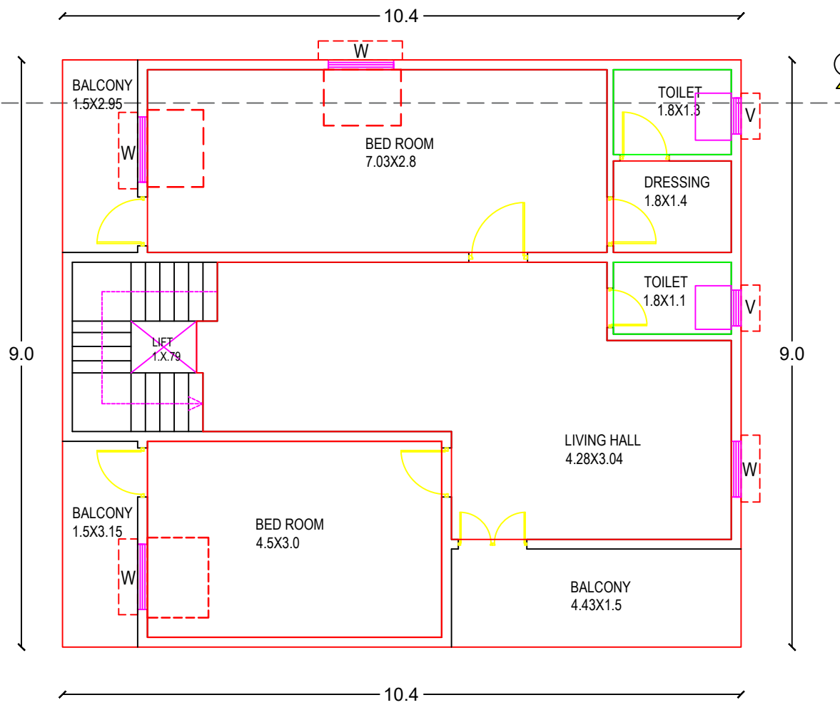
PRO.SECOND FLOOR PLAN SCALE:1:100
