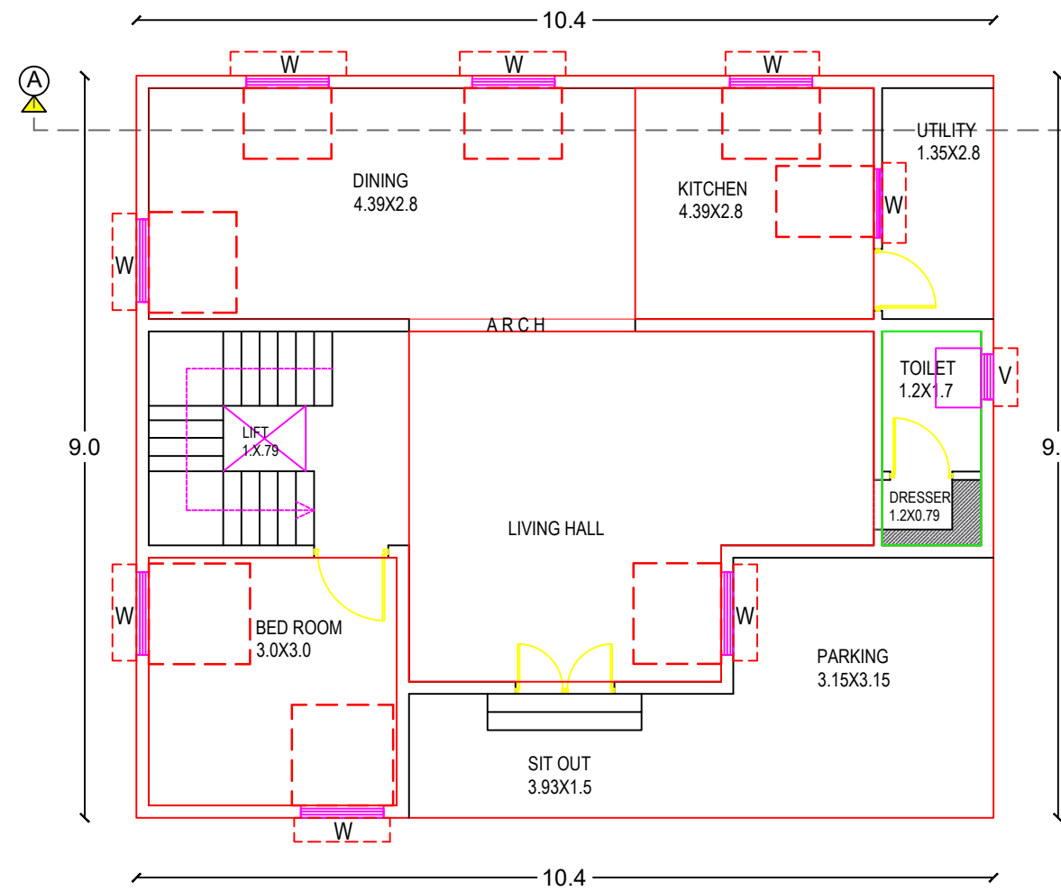
PRO.GROUND FLOOR PLAN SCALE:1:100
