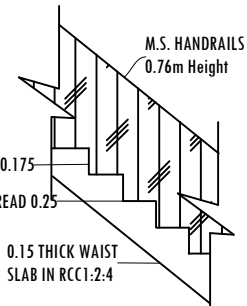
STAIRCASE DETAILS SCALE- 1:20
