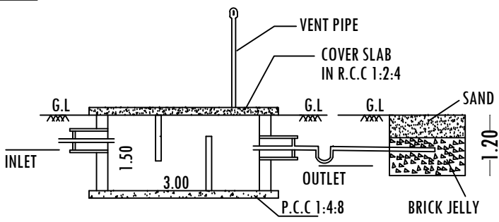
SECTION-AB
