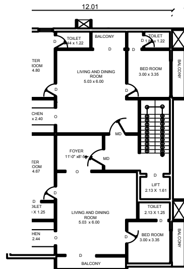
TYPICAL FIRST, SECOND & THIRD FLOOR PLAN
