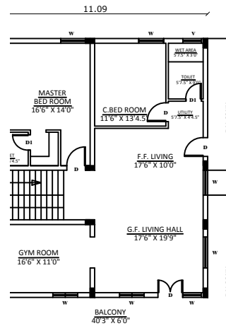
PROPOSED FIRST FLOOR PLAN DUPLEX
