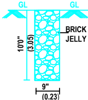
PERCOLATION PIT
