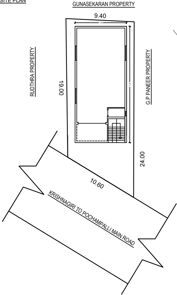
SITE PLAN
