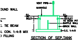
SECTION OF SEPTIC TANK
