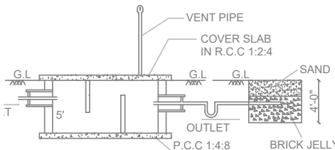
SECTION-AB
