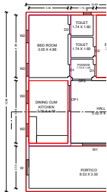
PRO. GROUND FLOOR PL
