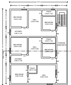
PRO. SECOND FLOOR PLAN
