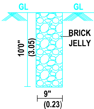
PERCOLATION PIT
