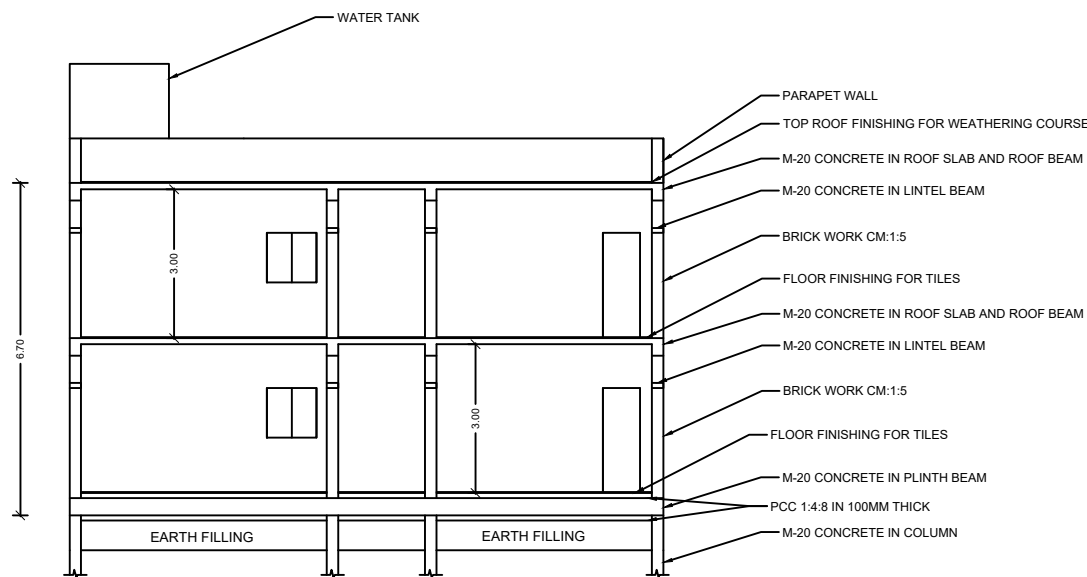
CROSS SECTION
