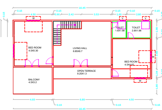
PRO.FIRTS FLOOR PLAN SCALE:1:100
