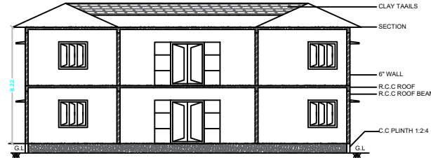
SECTION "A-B"
