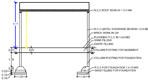
SECTION ON-AA
