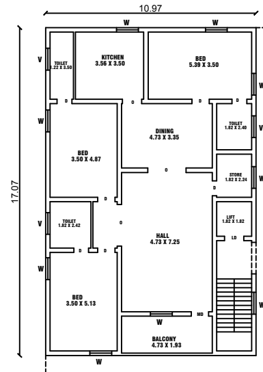
TYPICAL SECOND & THIRD FLOOR PLAN
