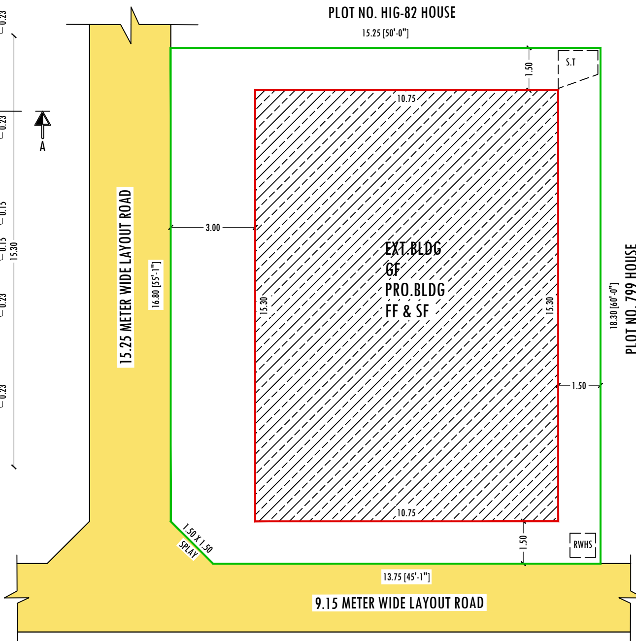
SITE PLAN
