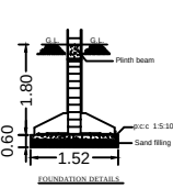
FOUNDATION DETAILS (NOT TO SCALE)
