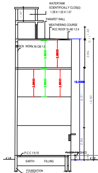
SECTION "A-B"
