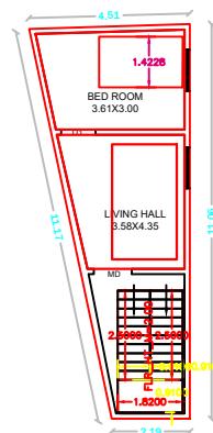
PRO. SECOND FLOOR (RESIDENTIAL).
