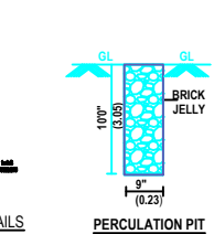
PERCOLATION PIT
