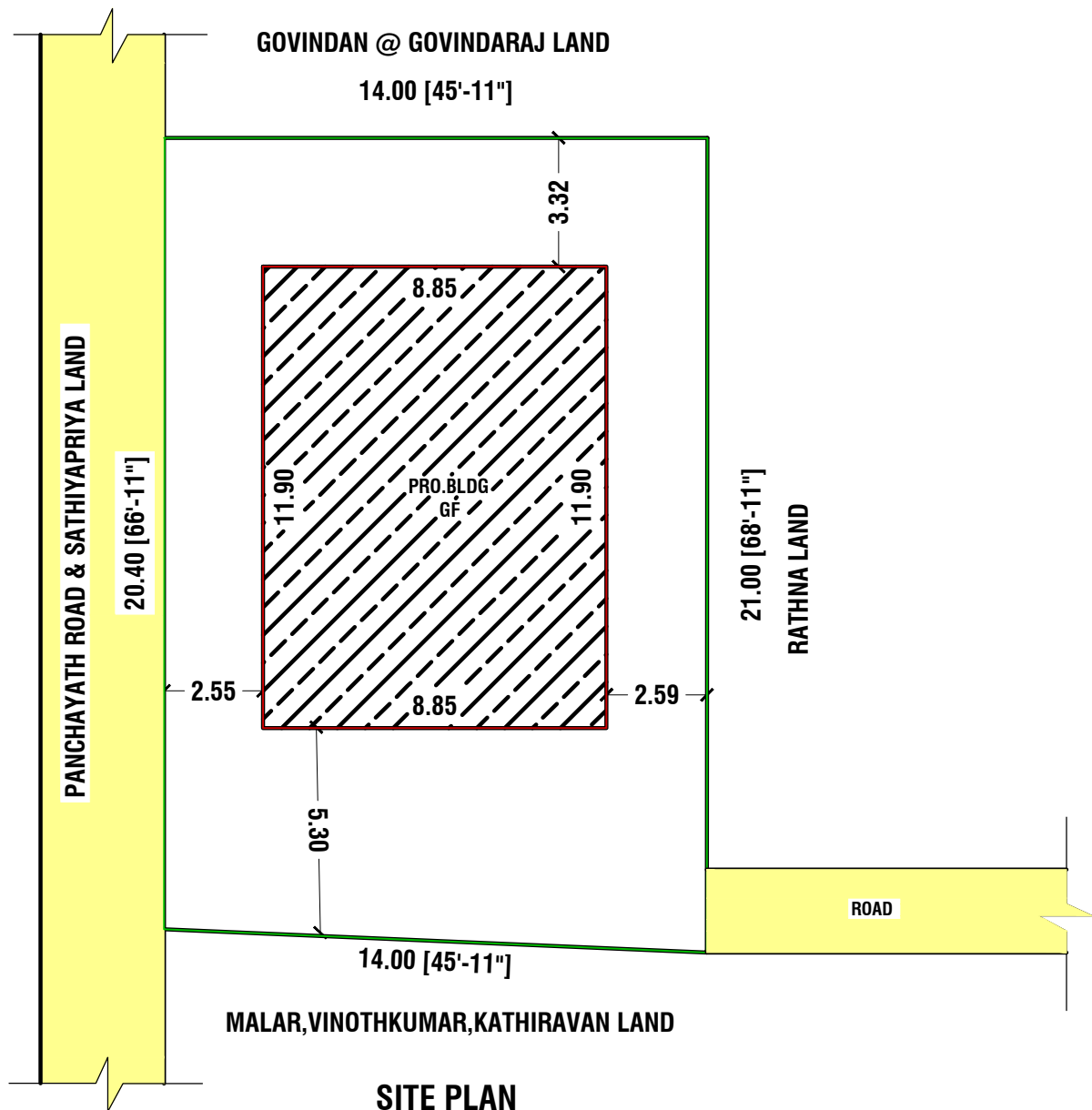
SITE PLAN
