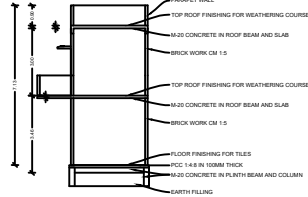
CROSS SECTION
