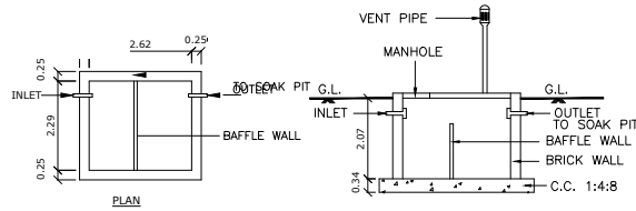
SECTION OF SEP.TANK
