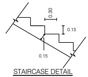
STAIRCASE DETAIL
