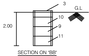
SECTION ON 'BB'
