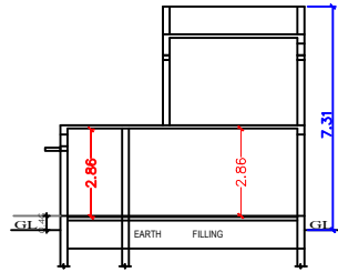
SECTION "B"
