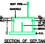
SECTION OF SEP.TANK
