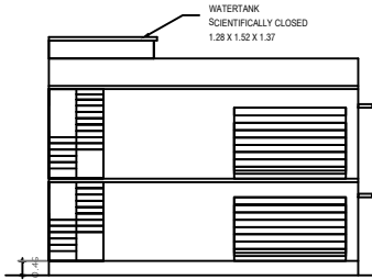
FRONT ELEVATION. AA
