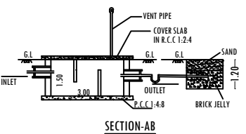
SECTION-AB
