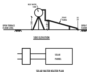
SOLAR WATER HEATER PLAN
