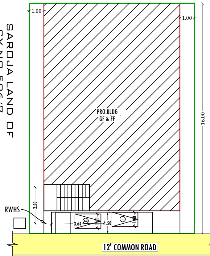
SITE PLAN
