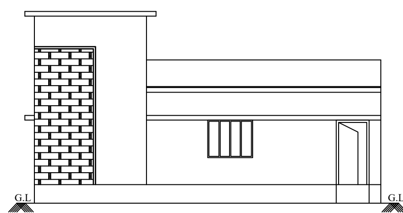
Elevation Plan
