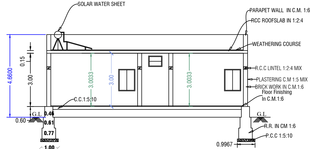
Section On-"AB"
