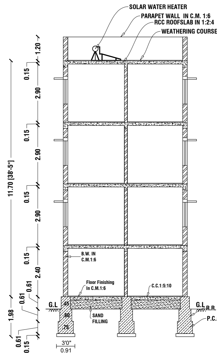
SECTION -AA
