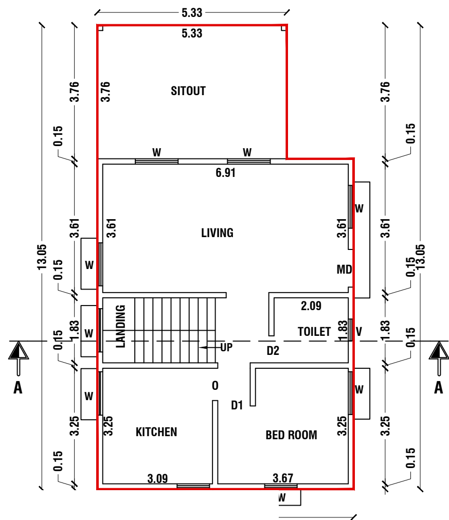
PLAN
