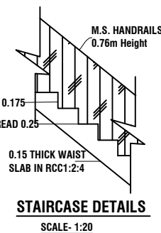
STAIRCASE DETAILS SCALE- 1:20
