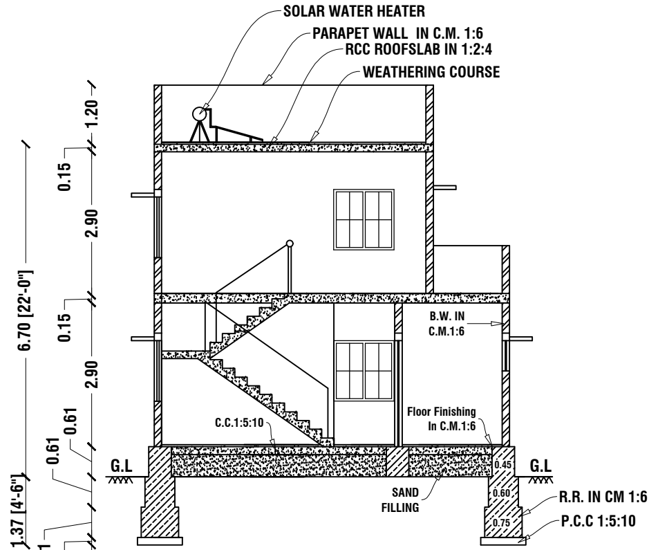
SECTION-AA
