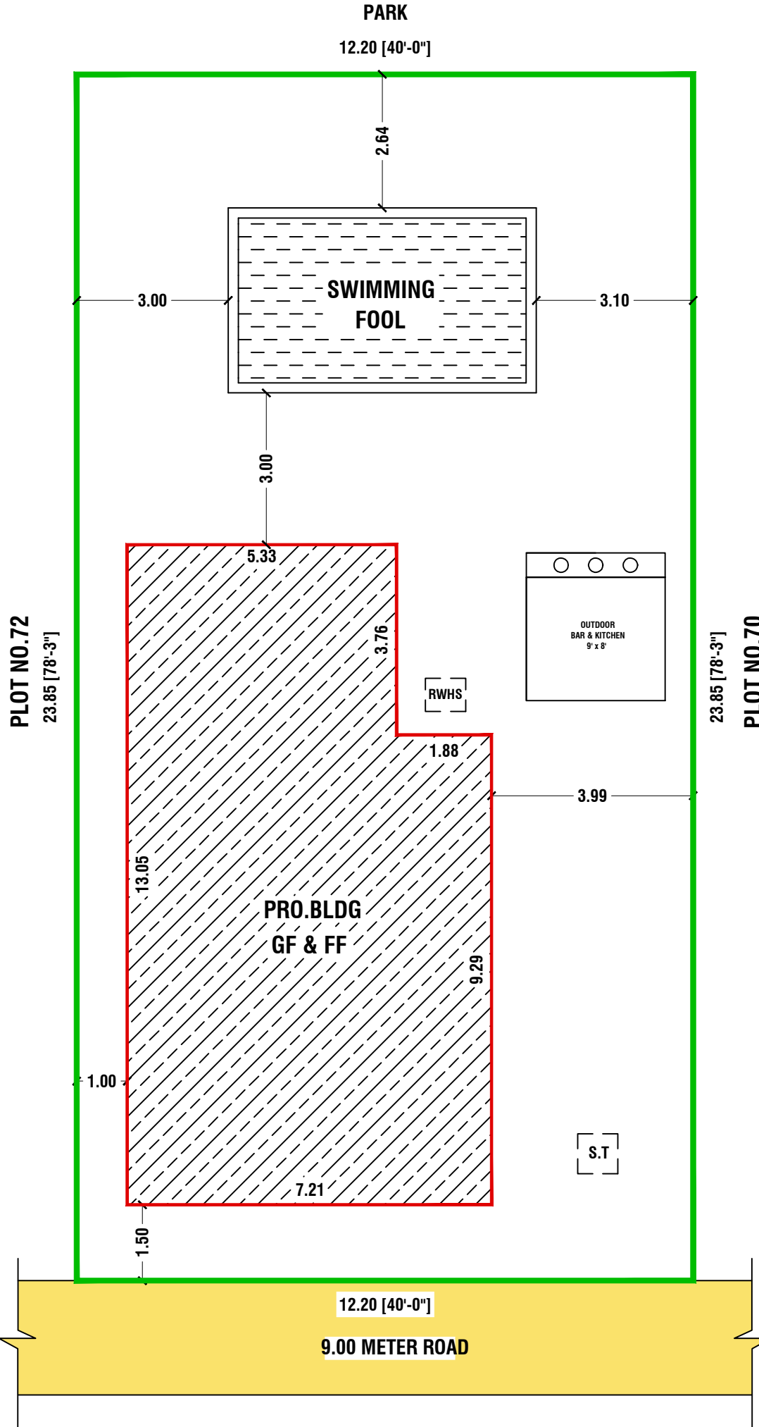
SITE PLAN
