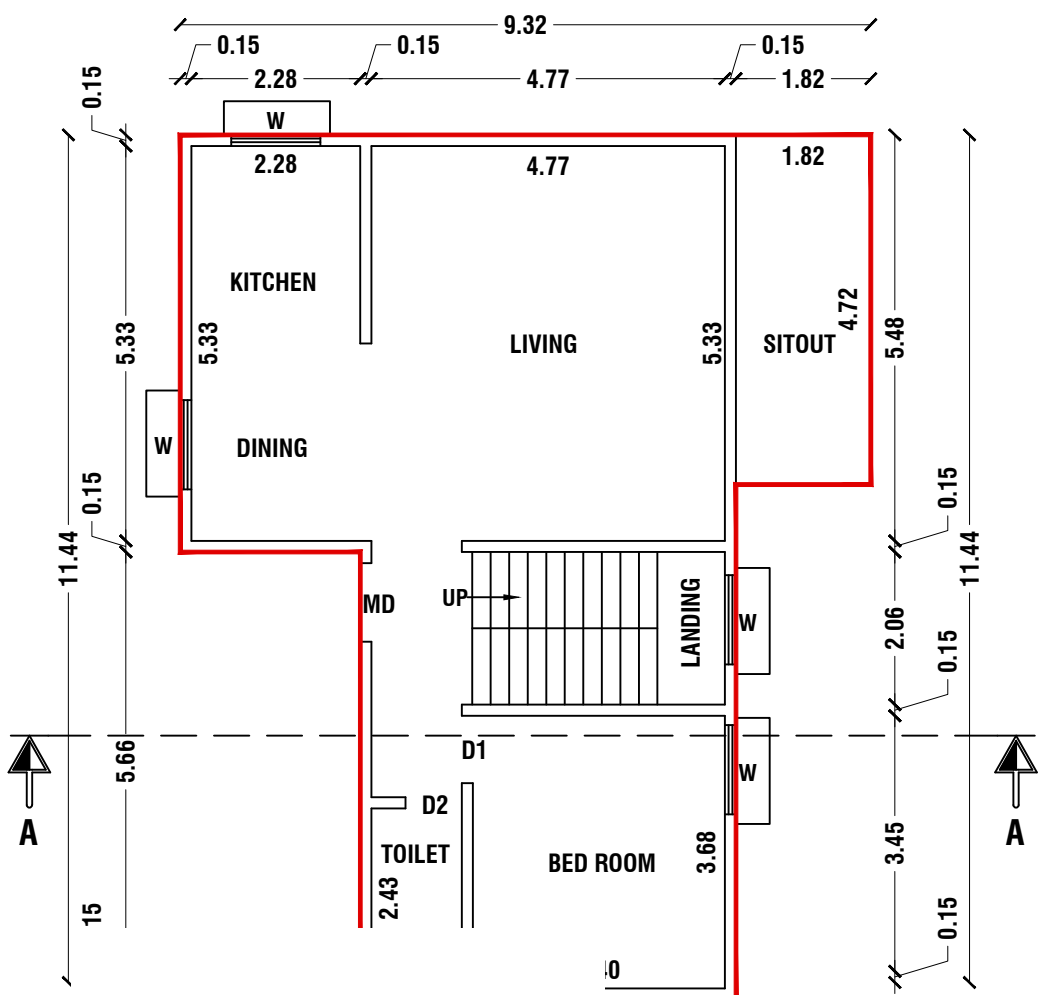
GR PLAN
