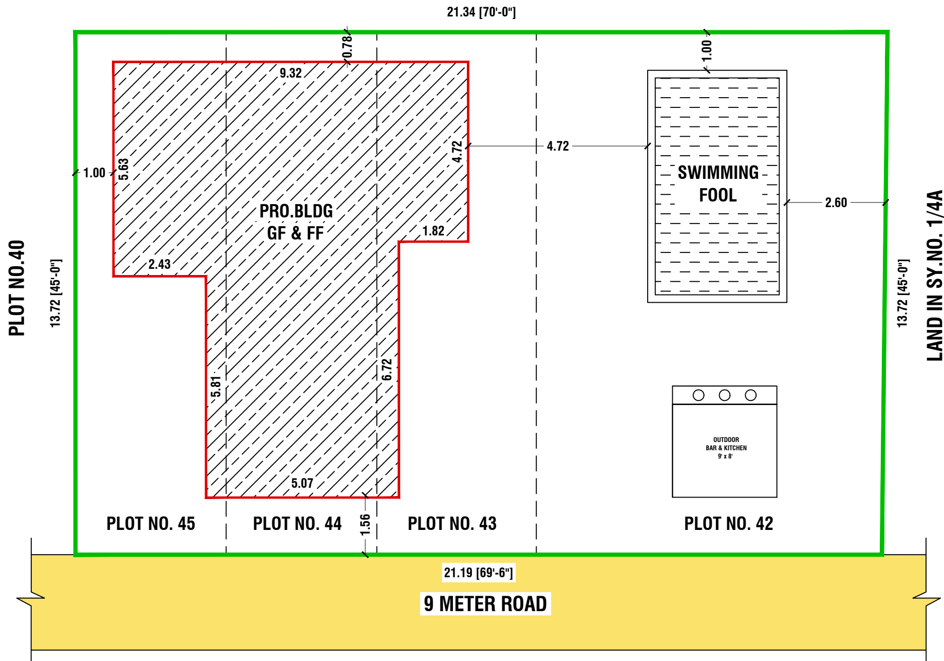
SITE PLAN
