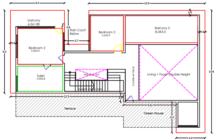
PRO.FIRST FLOOR PLAN SCALE:1:100
