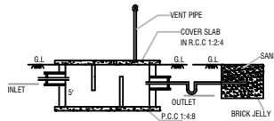
SECTION-AB
