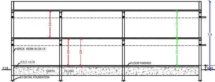
SECTION "A-B"
