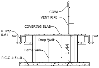
SECTION ON JS
