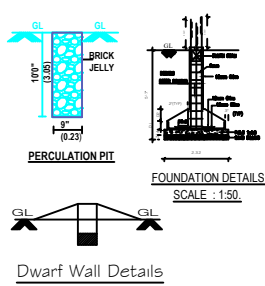
Dwarf Wall Details
