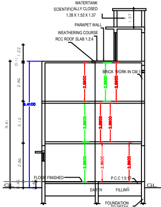
SECTION "A-B"
