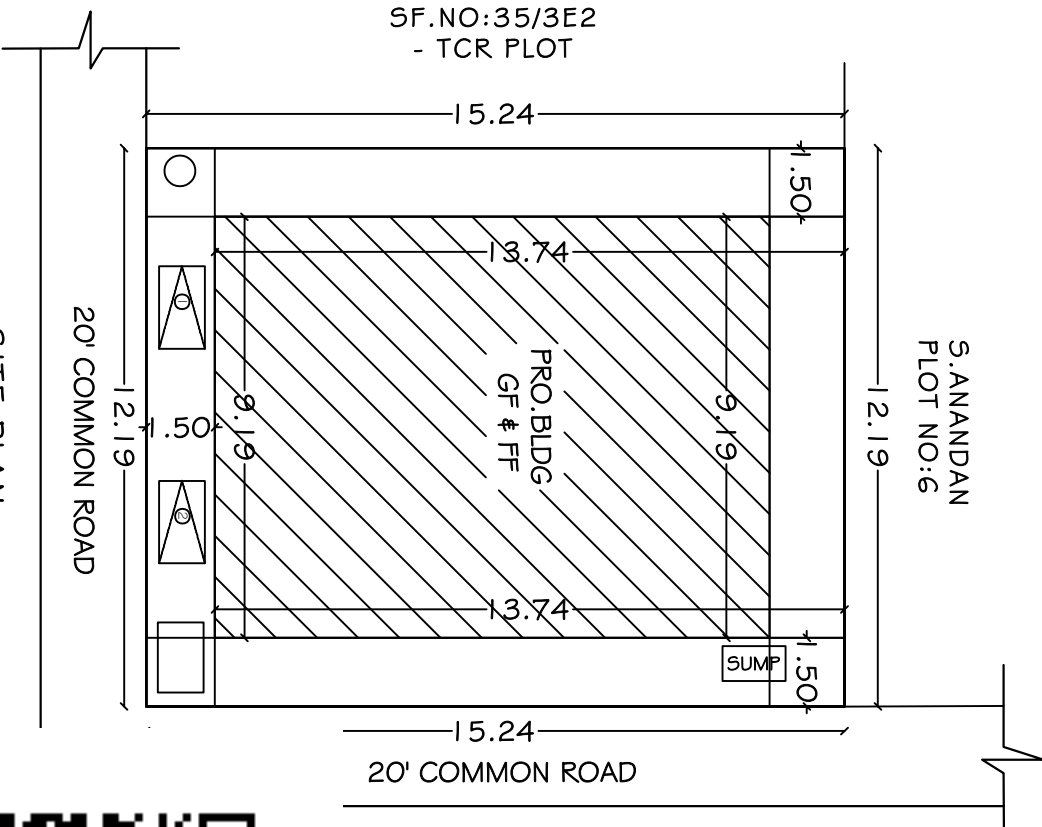
SITE PLAN
