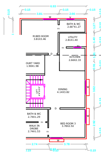
1. FIRST FLOOR PLAN SCALE: 1:100
