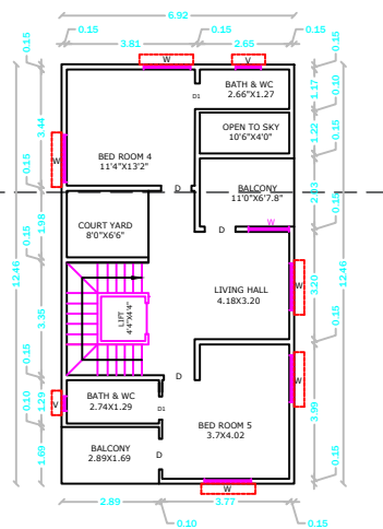
PRO.SECOND FLOOR PLAN SCALE:1:100
