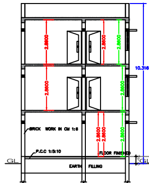
SECTION "A-B"
