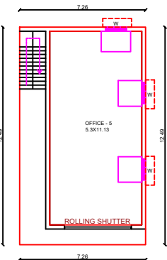
GROUND FLOOR (COMMERCIAL)
