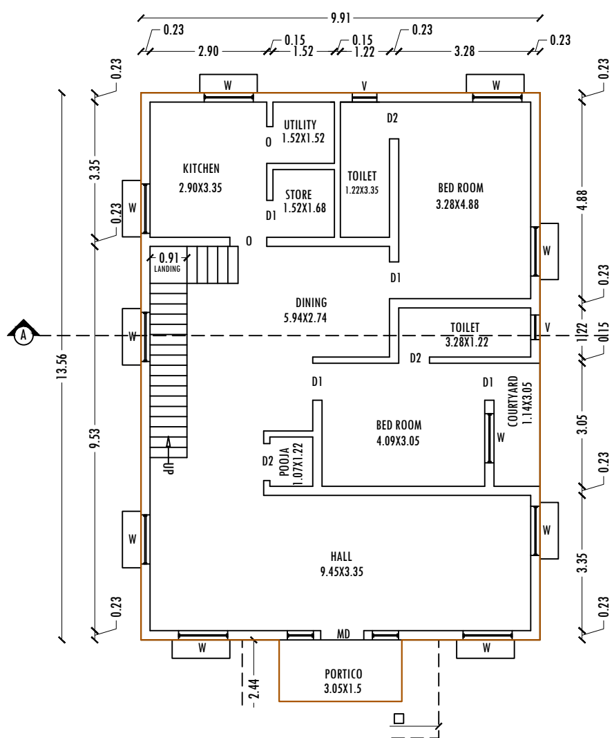
R PLAN
