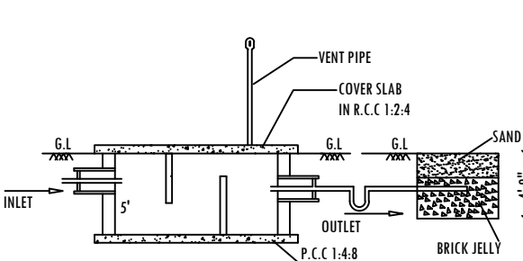
SECTION-AB
