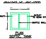
PLAN SEPTIC TANK
