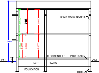
SECTION "A-B"
