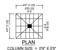
COLUMN SIZE = 0'9" X 0'9"
