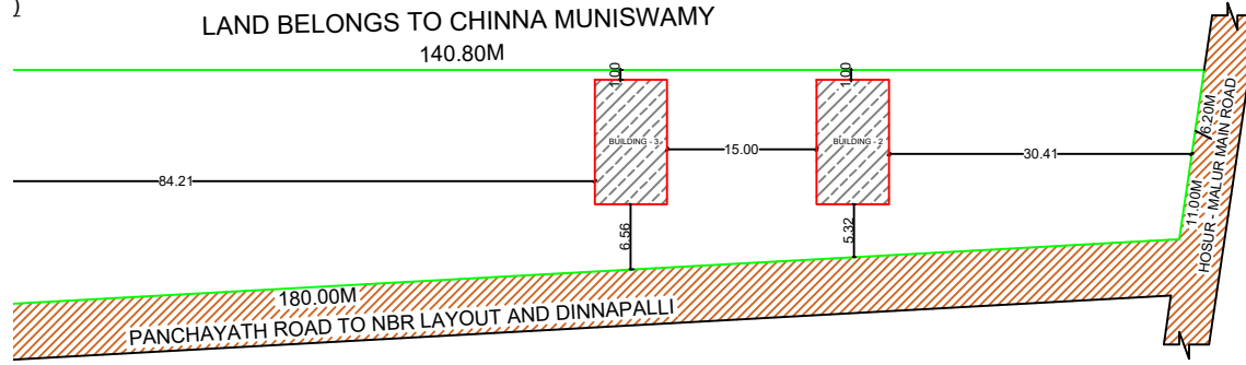
SITE PLAN
