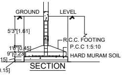
FOUNDATION DETAILS
