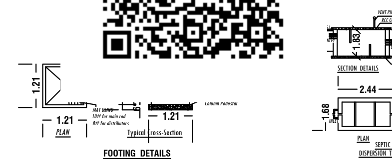
FOOTING DETAILS
