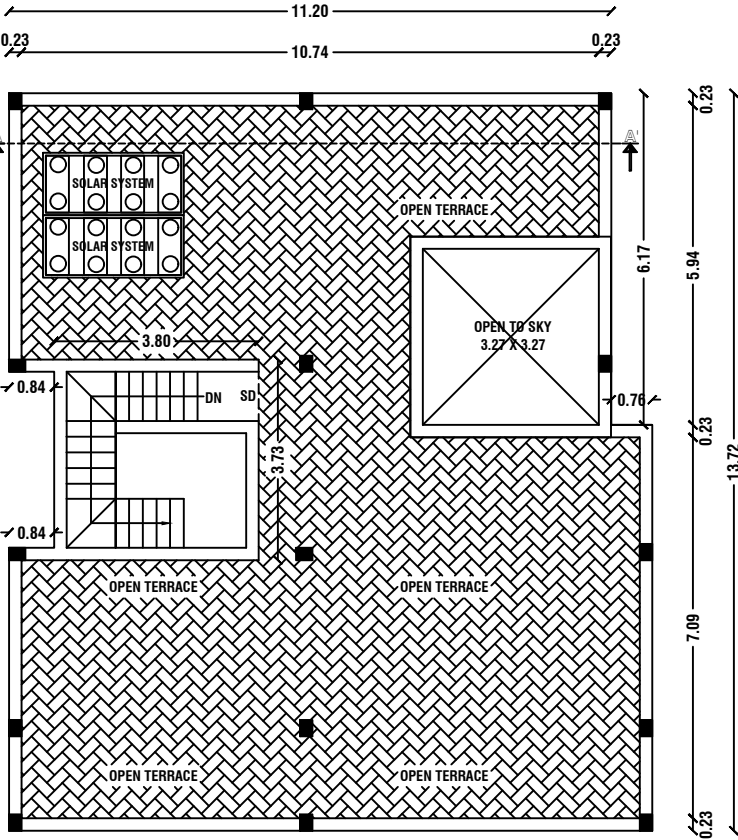
HEAD ROOM CUM OPEN TERRACE FLOOR PLAN
