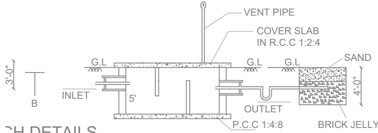
SECTION-AB
