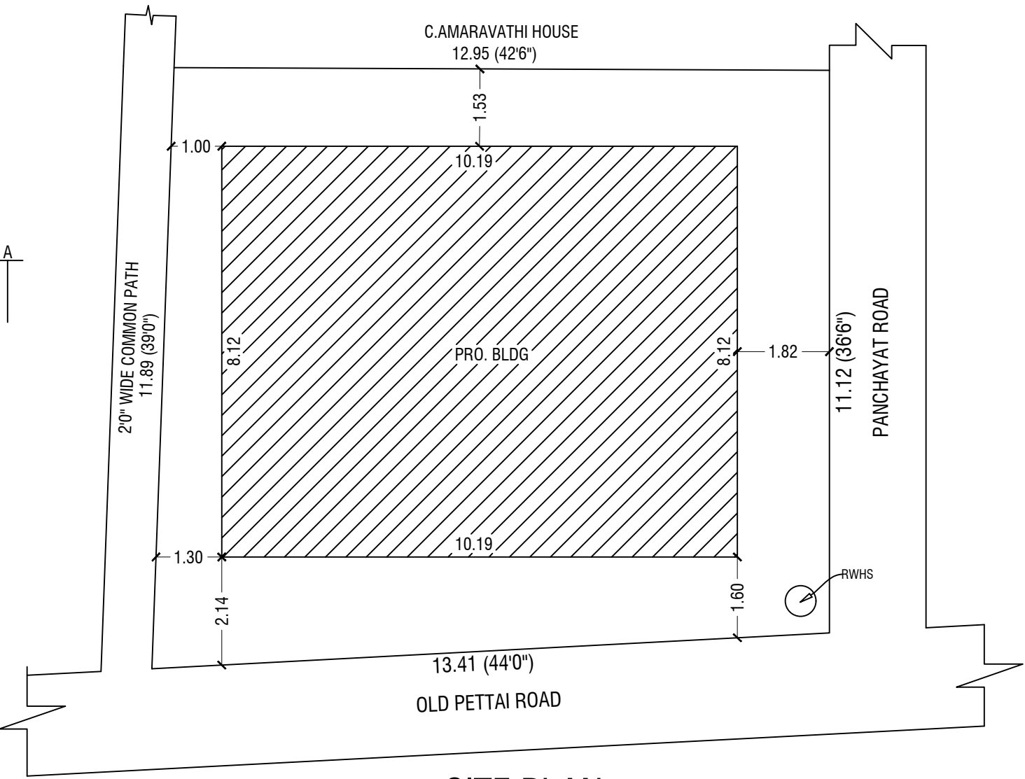
SITE PLAN
