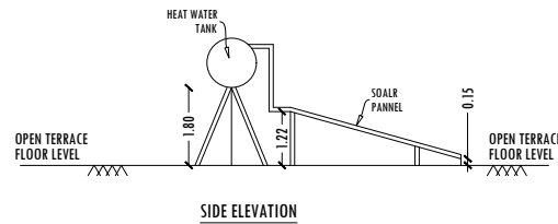
SIDE ELEVATION SOLAR WATER HEATER PLAN
