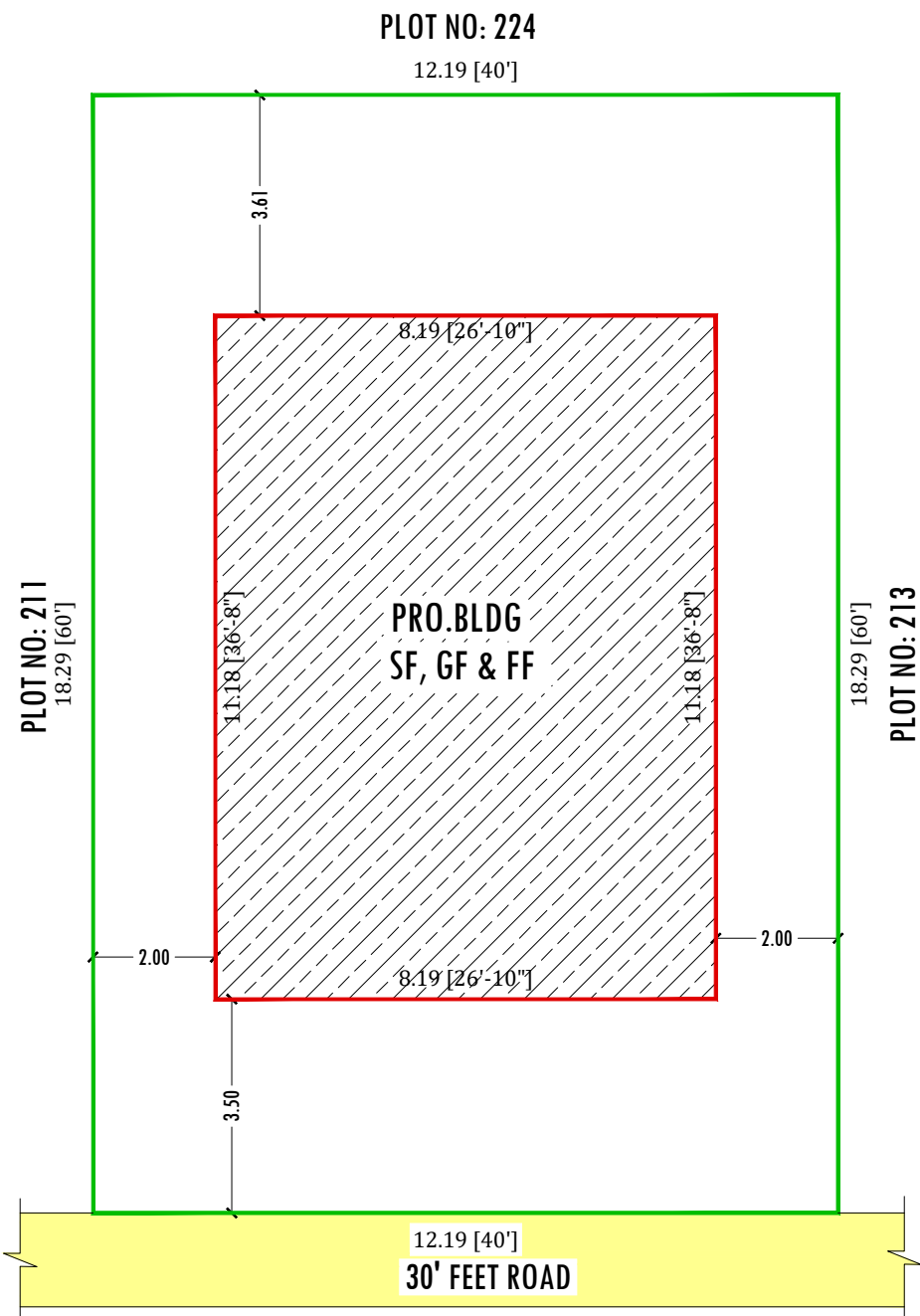
SITE PLAN
