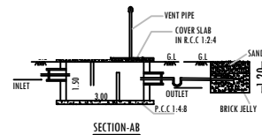
SECTION-AB
