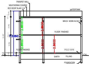
SECTION "A-B"
