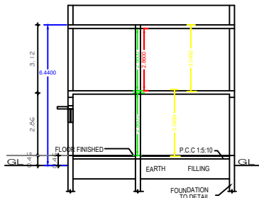
SECTION "A-B"
