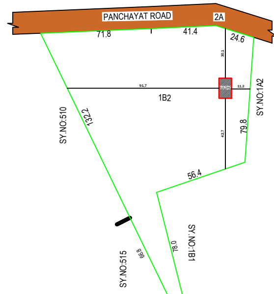
SITE PLAN
