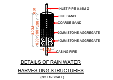
DETAILS OF RAIN WATER HARVESTING STRUCTURES
