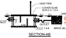
SECTION-AB
