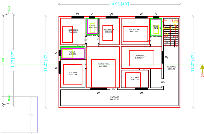
PRO.FIRST FLOOR PLAN
