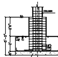
FOOTING DETAIL
